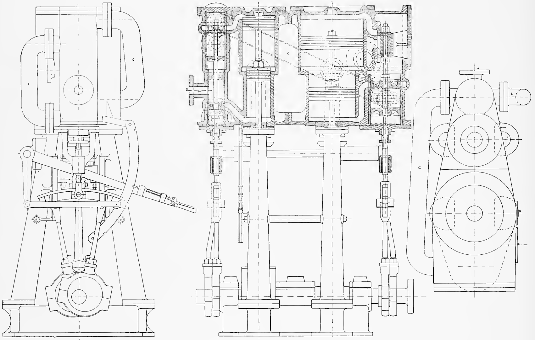
LUMGAIR'S PATENT QUADRUPLE-EXPANSION MARINE ENGINE.—Designed by David Lumgair, West Bay City, Mich.
